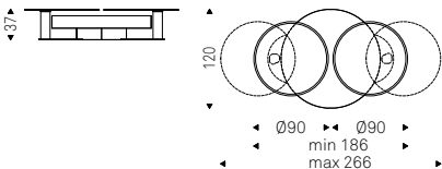
Arena Double Bond
